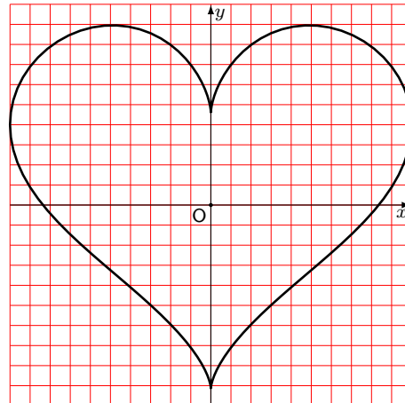
Figure 13: A heart shaped mathematical function drawn with a thinly sampled piecewise continuous line
