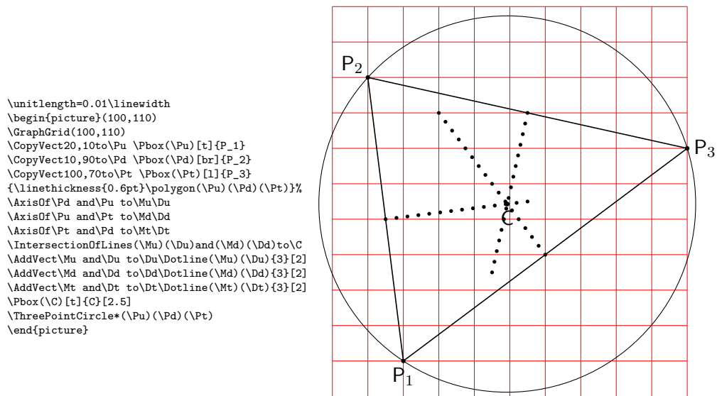
Figure 21: Determination of the circumcenter and of the circumcircle
