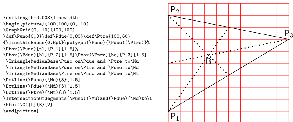
Figure 18: Determination of the barycenter
