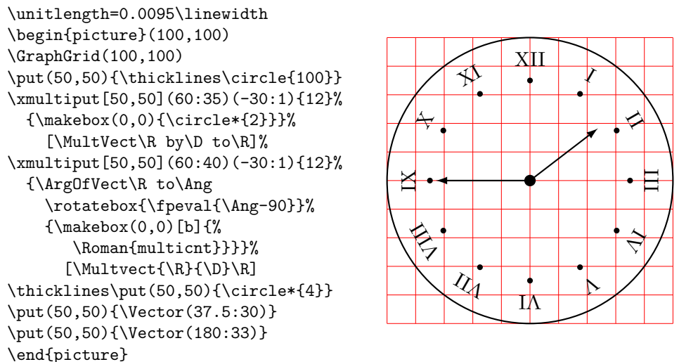
Figure 11: Usage example of the \xmultiput command
