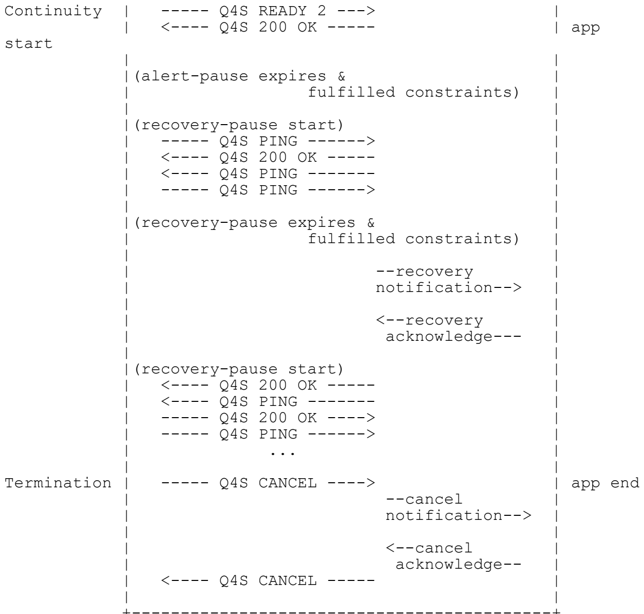
Figure 4 Reactive alerting mode.
