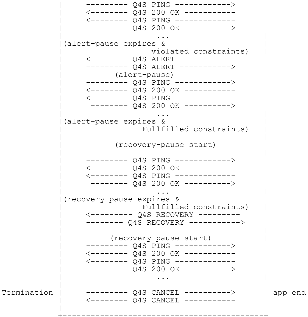
Figure 3 Q4S-aware-network alerting mode.
