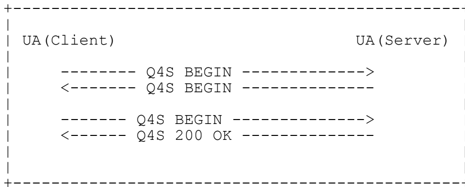
Figure 15 P2P roles.
