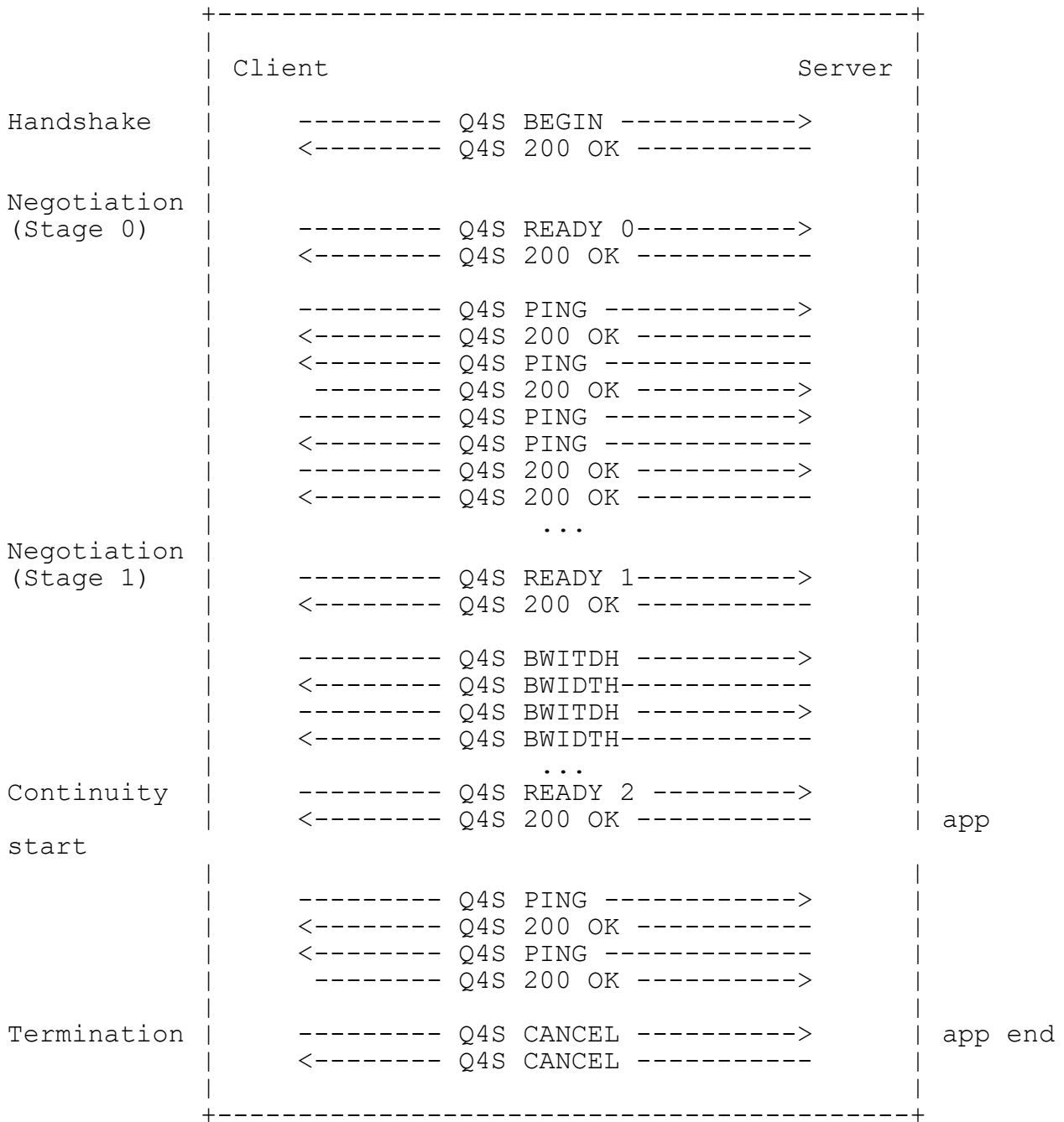
Figure 2 Successful Q4S message exchange.
