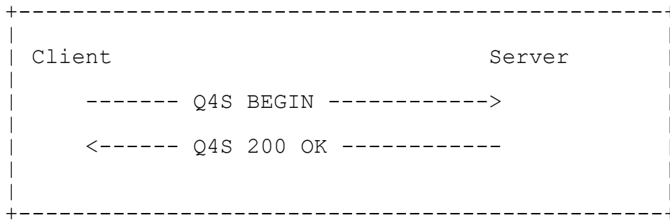
Figure 7 Handshake phase.
