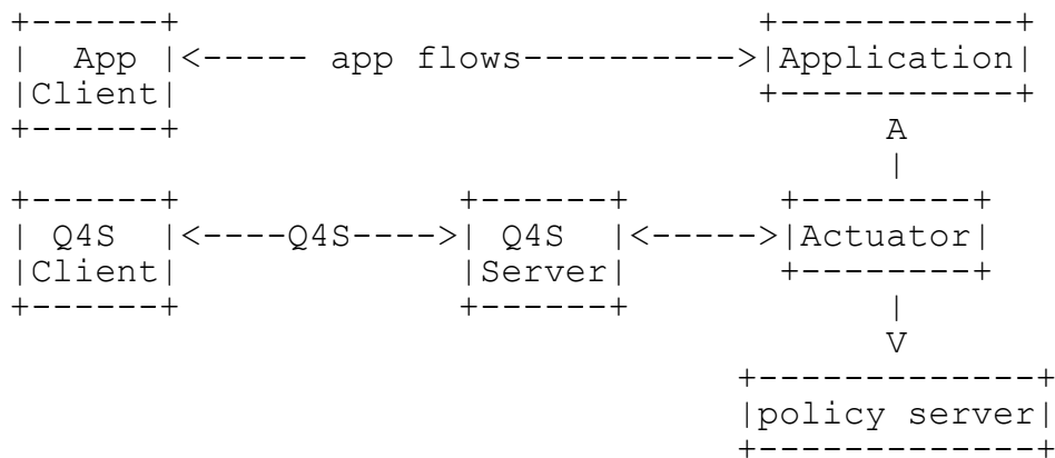
Figure 1 Reactive scenario
